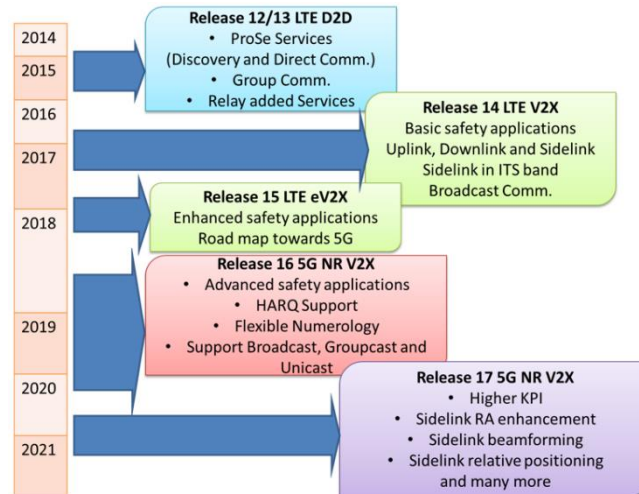
Figure 1. 3GPP Releases timeline Sidelink D2D communication
