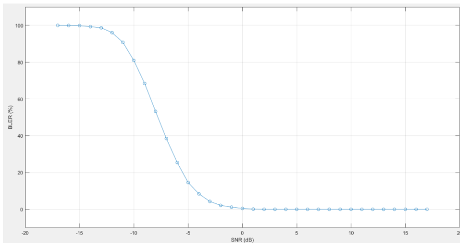
Figure 7. BLER Vs. SNR for SCI
