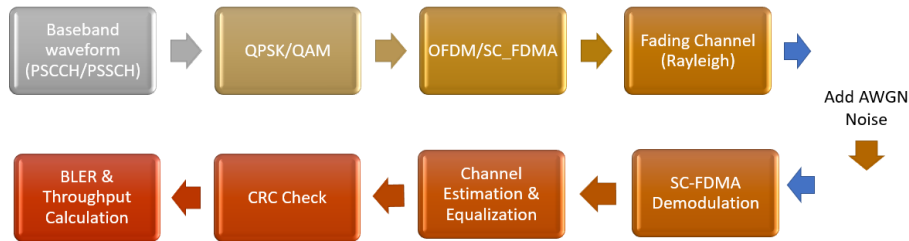
Figure 5. Block Diagram for Sidelink information transmission and reception
