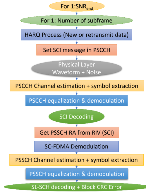
Figure 6. Flow chart represents sidelink transmission and reception
