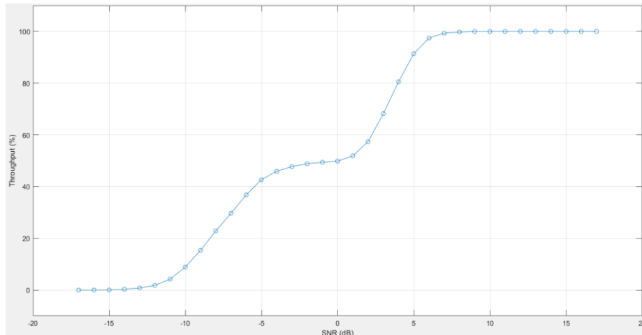
Figure 8. Throughput Vs. SNR for SL-SCH (sidelink data)
