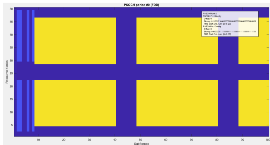
Figure 3. PSCCH, SCI and PSSCH period
