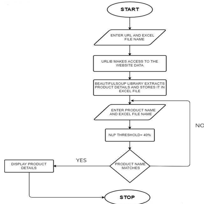
Figure 4. Flow chart of the task Web Scrapping Using Python Applied on Flipkart
