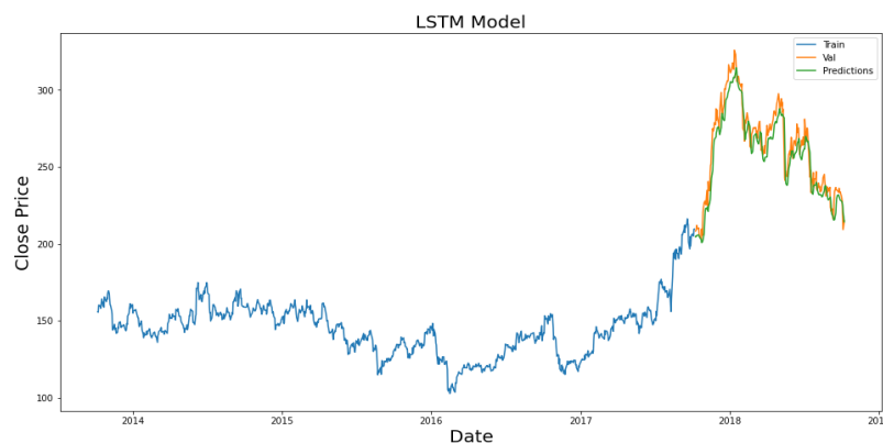
Figure 5. Predicted Value - Actual Value result 1 (With less epox value)
