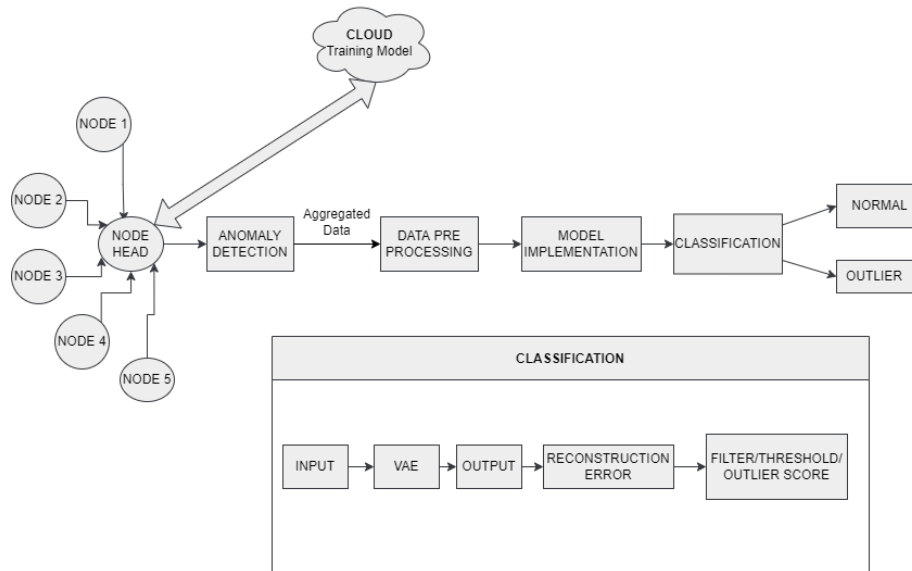
Figure 6. Proposed Model
